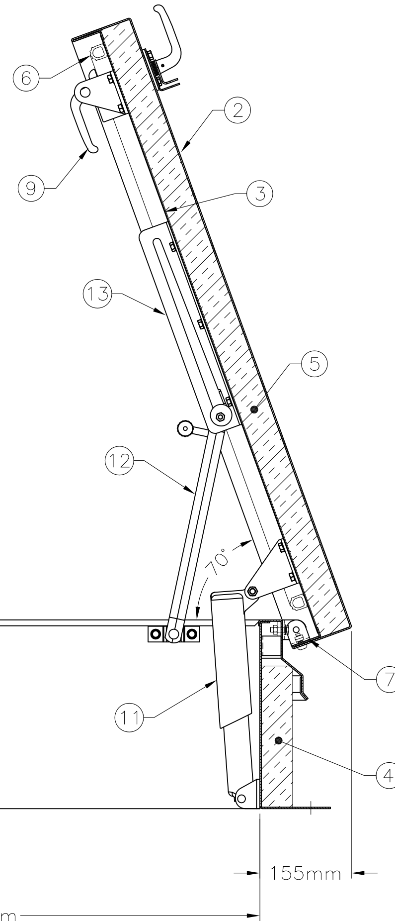
SECTION
