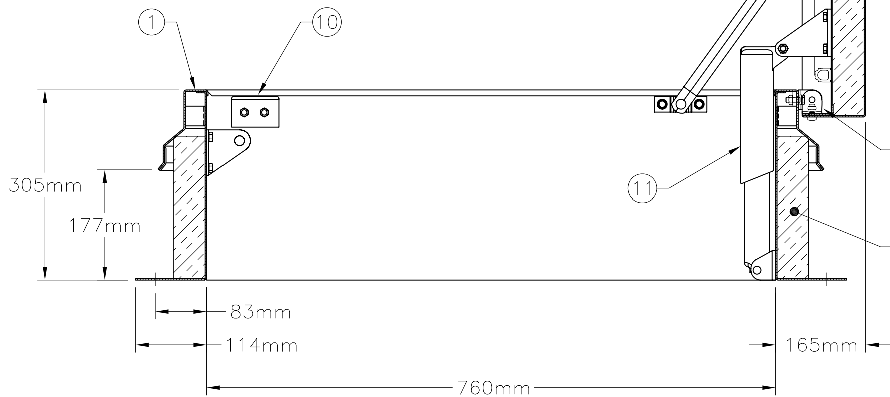
SECTION
