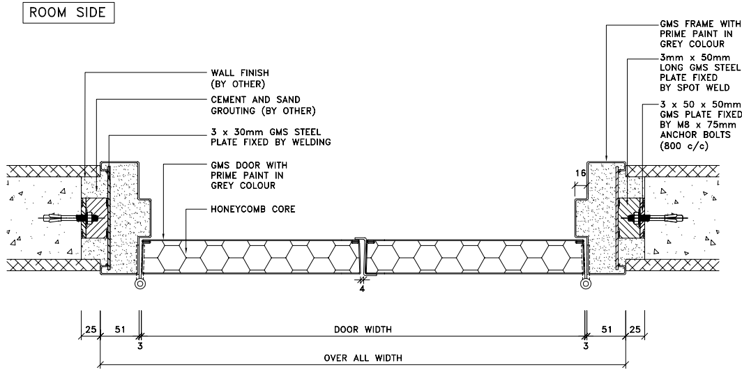
(DOUBLE DOOR LEAVES-FIXING DETAIL) SECTION B2 - B2
