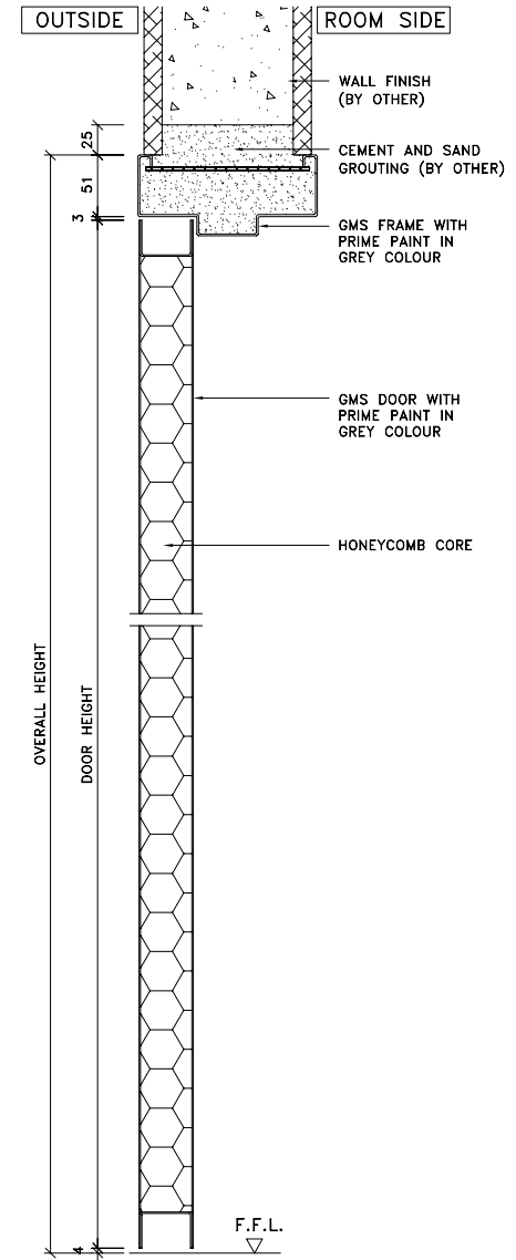
(TOP & BOTTOM DETAIL) SECTION A2 - A2
