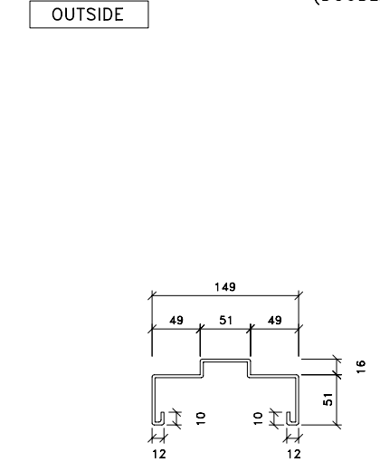
GMS FRAME SECTION DETAIL
