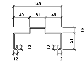
GMS FRAME SECTION DETAIL
