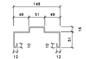
GMS FRAME SECTION DETAIL
