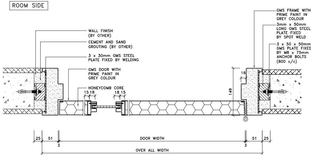
(SINGLE DOOR LEAF-FIXING DETAIL WITH GLAZING PANEL)
