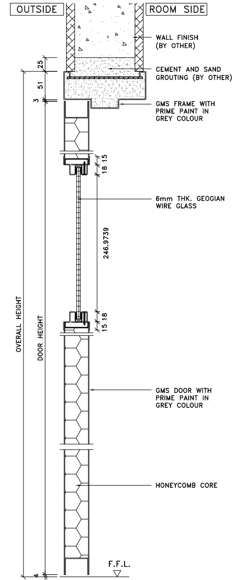
(TOP & BOTTOM DETAIL)
