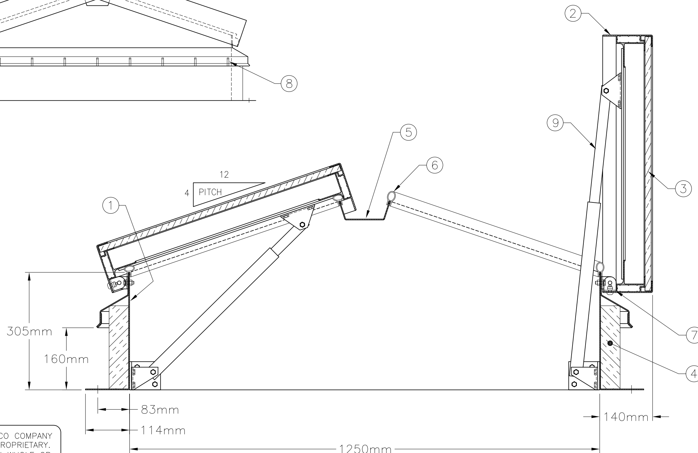
SECTION
